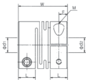
Type SRBM - □□C
