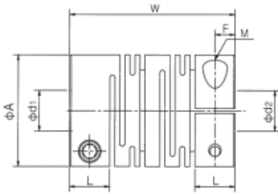
Type SRB - □□ (Aluminium) Type SRBS - □□ (Inox)
