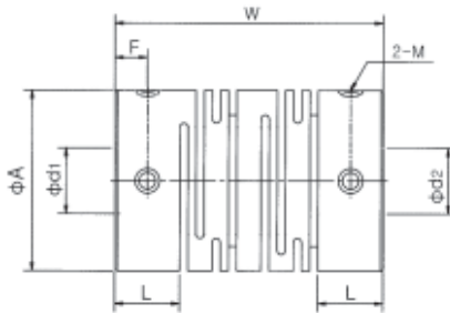
Type SRB - □□C (Aluminium) Type SRBS - □□C (Inox)
